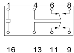
TERMINAL ARRANGEMENT (BOTTOM VIEW)
